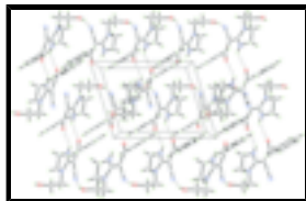
Fig. 2. Packing diagram for (I), viewed down the b axis with hydrogen bonds indicated by dashed lines.
